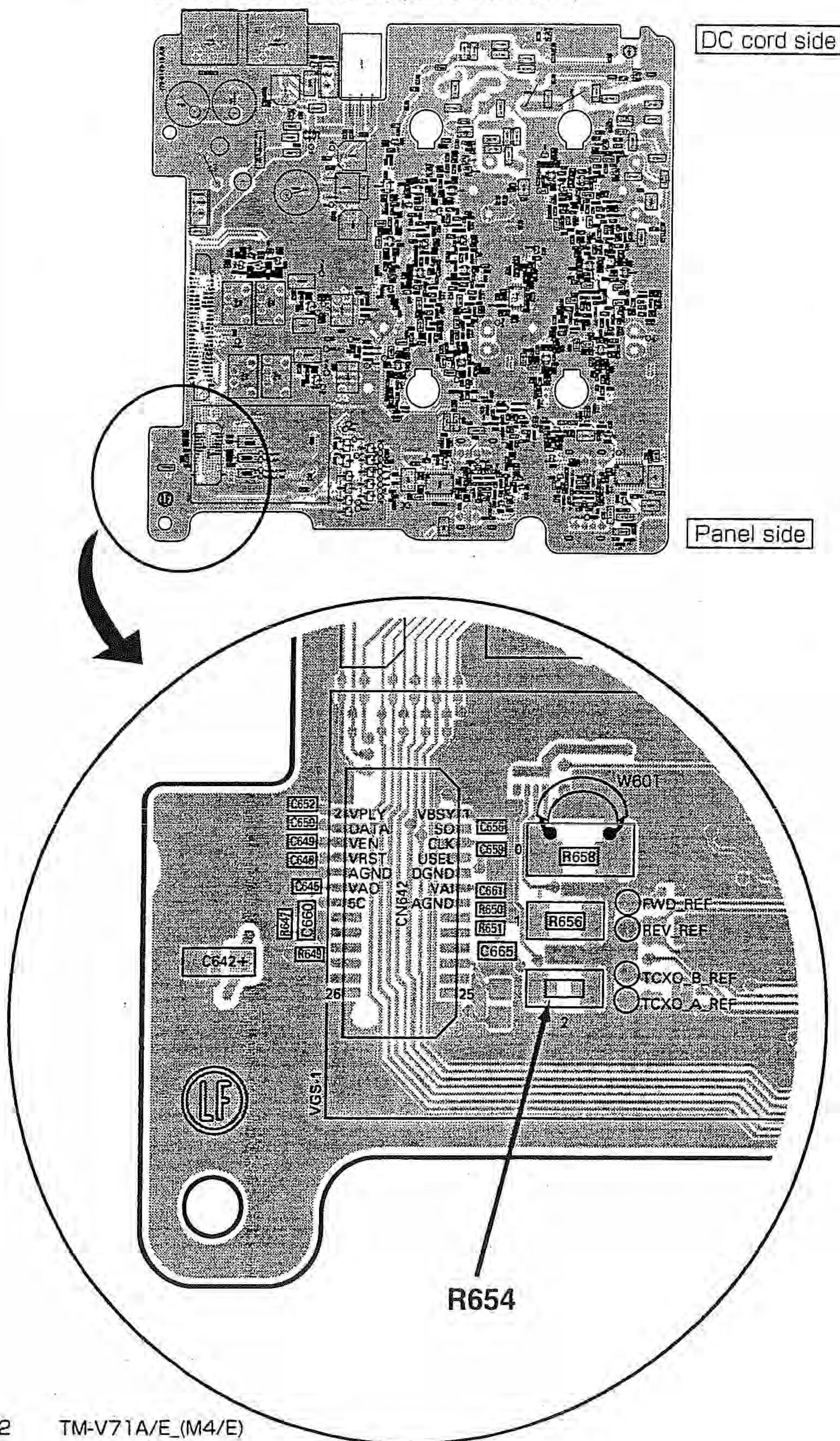
TX-RX unit x57-731 A/6 (Component side)
