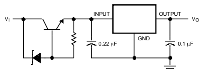
Figure 29. High Input Voltage Circuits
